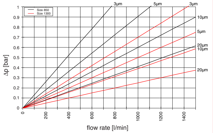
BN3HC: Element sizes 1700 / 2600
